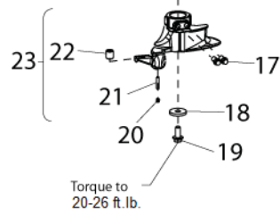
Steel DuckHead® Mount/Demount Tool
